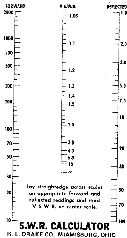
Figure 3-3. SWR Nomograph
