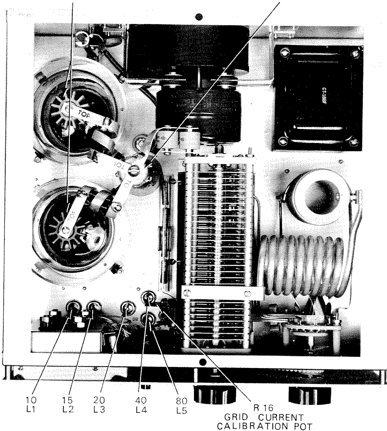
Figure 5-1. Component Locations, Top View
